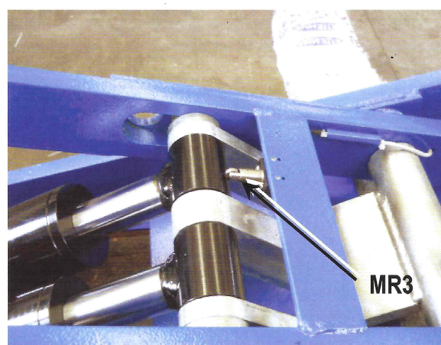
Pic. 24 P2 cylinder position sensing micro
