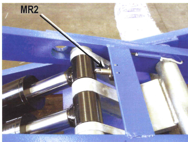
Pic. 23 P1 cylinder position sensing micro
